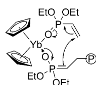
Scheme 3. Postulated DEVP intermediate in the group-transfer mechanism.
